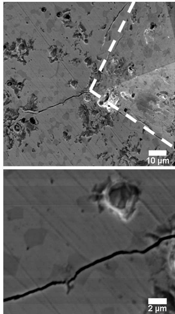
Fig. 10. SEM of an indent (10 kg load) in 8:1 ceramics pressureless sintered at 1900 °C (dashed line shows the corner of the indent).
