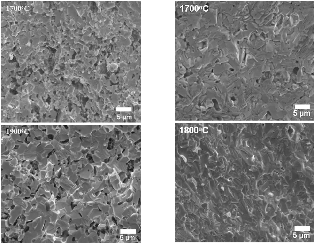
Fig. 7. SEM of 4:1 ceramics prepared by pressureless sintering at 1700 and 1900 °C for 2 h in He.
