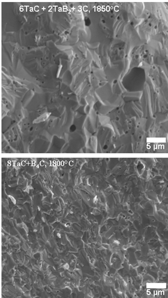
Fig. 9. SEM of TaC–TaB 2 –C ceramics prepared from 8TaC + B 4 C (reactive) and from 6TaC + 2TaB 2 + 3C (non-reactive) mixtures by pressureless sintering.
